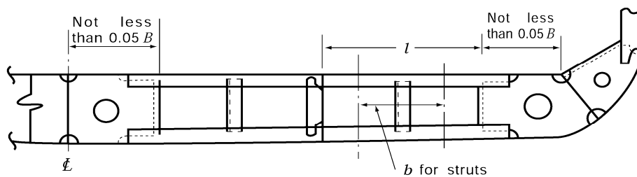
Fig 10.7.1 Open Floors
