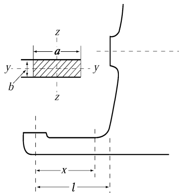
Fig 10.2.1 Shoe piece
